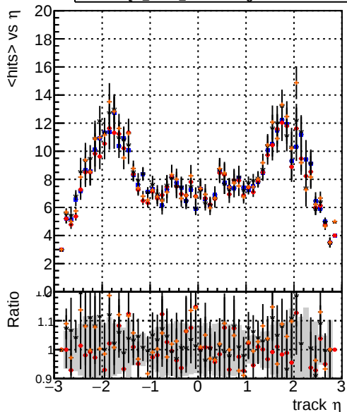
Legend: DQM_mkFit_TToriginal (blue line), DQM_mkFit_TTNEWnoMS-genMatch-chi200 (red line), DQM_mkFit_TToriginal-106 (black line), DQM_mkFit_TTNEWMS-genMatch-chi200 (orange line) mean hit
