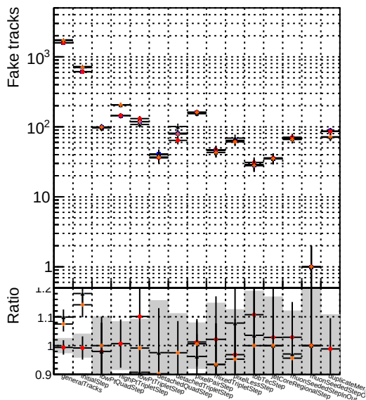
Number 1 DQM_mkFit_TTNEWMS-genMatch-chi200 2 DQM_mkFit_TToriginal-106 3 DQM_mkFit_TTNEWMS-genMatch-chi200
