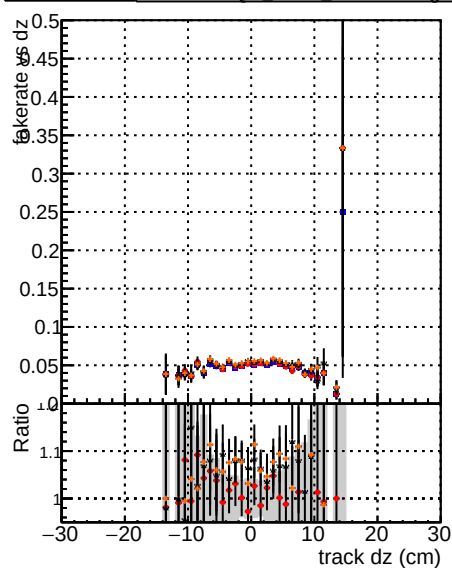
Fake rate vs dz Legend: DGM (black), mkt (blue), Fit (red), T (green), Original (grey), genMatch-chi200 (orange)
