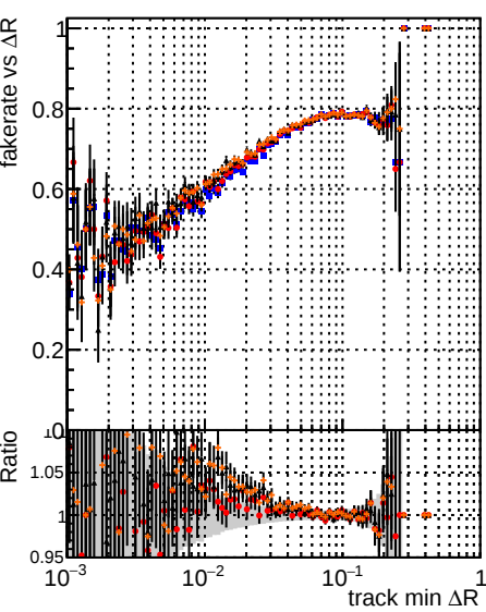
Fake rate vs \Delta R(\text{track, jet}) Legend: DOM mktFit T-Original DOM mktFit T-NEWMS-genMatch-chi200 DOM mktFit T-NEWMS-genMatch-chi200
