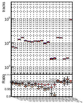
N of reco track vs. s DGM mkrItt -- NEWMS-genMatch-chi200 DGM mkrItt -- original-106 DGM mkrItt -- NEWMS-genMatch-chi200
