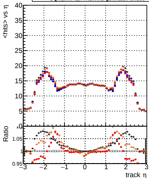
mean hit DQM_mkFit_TToriginal DQM_mkFit_TTNEWnoMS-genMatch-chi200 DQM_mkFit_TToriginal-106 DQM_mkFit_TTNEWMS-genMatch-chi200
