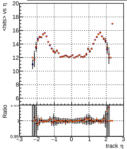
mean hit DQM_mkFit_TToriginal DQM_mkFit_TTNEWnoMS-genMatch-chi200 DQM_mkFit_TToriginal-106 DQM_mkFit_TTNEWMS-genMatch-chi200
