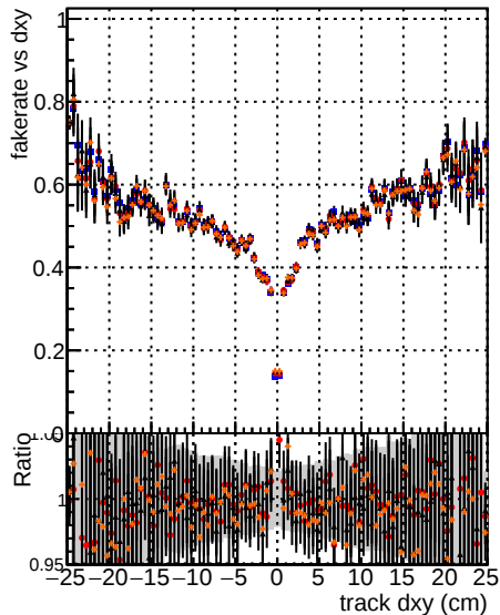
Legend for Fake rate vs dxy and Duplicates Rate vs Dxy plots: DOM (black line) mkt (blue line) fit (orange line) T (green line) Original (red line) REWM (purple line) genMatch (brown line) chi200 (pink line)
