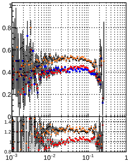
Fake rate vs \epsilon Legend: DOM CKE DOM mKEfit BDT CKEfit BDT mKEfit
