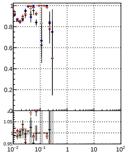
Legend for Fake rate vs v: DOM (black) CKE (red) BDT (blue) mKEit (orange)
