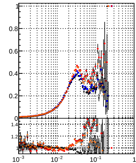
Fake rate vs \epsilon Legend: DOM CKE BDT mKEFit BDT mKEFit
