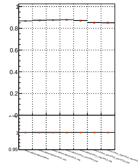
Fake rate vs. DOM SKE BDT-mkFit BDT-mkFit DOM SKE BDT-mkFit BDT-mkFit
