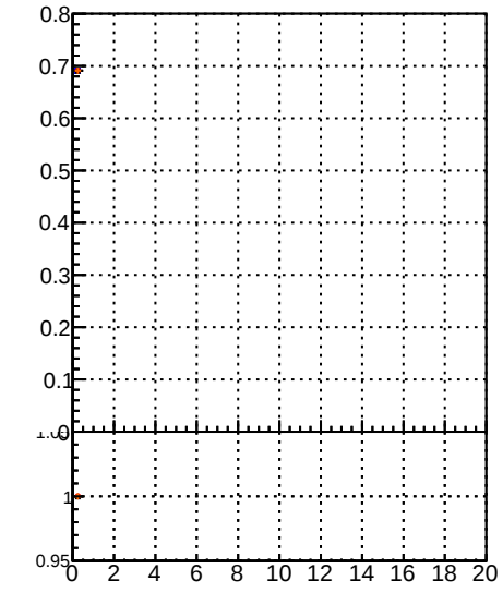
Fake rate vs. DOM SKE BDT-mkFit BDT-mkFit DOM SKE BDT-mkFit BDT-mkFit
