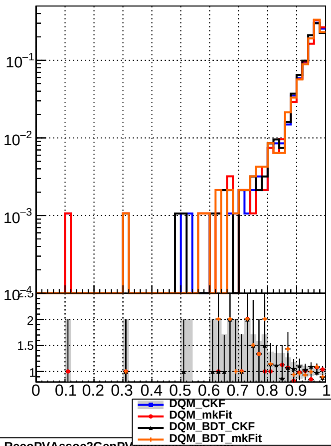
RecoPVAssoc2GenPVMatched_missing
