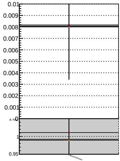
Fake rate vs. BQM SKE BQM-BDT BQM-BDT-mKFit
