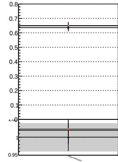
Fake rate vs. BQM SKE BQM-BDT BQM-BDT-mKFit
