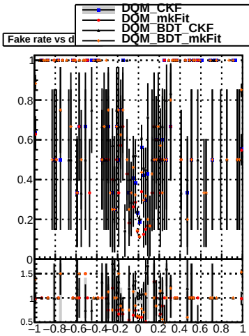
Fake rate vs dzpv
