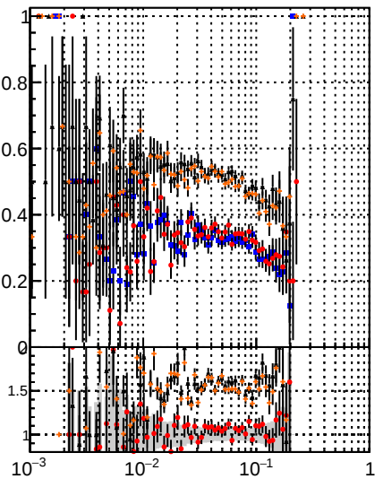
Fake rate vs \epsilon Legend: DOM CKE DOM mKEfit DOM BDT BDT mKEfit
