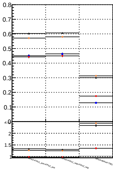
Fake rate vs. BGM SKE BGM BDT mKF
