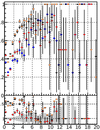
Fake rate vs. BGM SKE BGM BDT mKF
