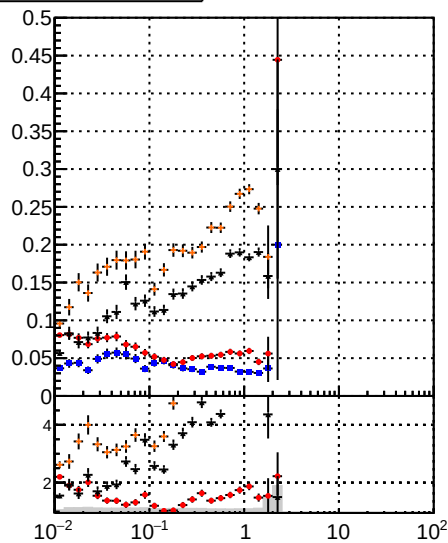
Legend: DOM CKE BDT mKEFit BDT mKEFit
