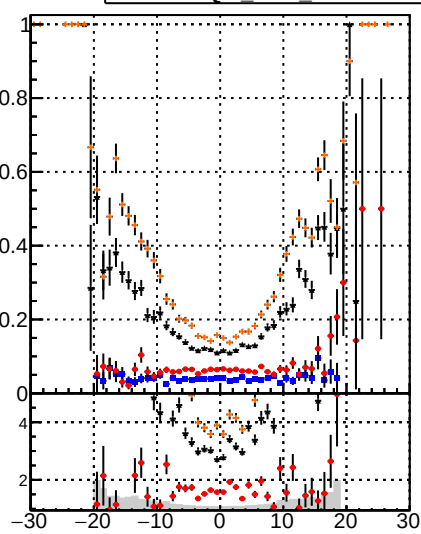
Legend: DOM CKE BDT mKEFit BDT mKEFit
