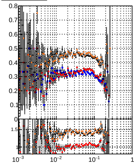
Fake rate vs \epsilon Method Color Symbol DOM Black Line CKE Blue Star mKEit Red Star BDT Orange Star
