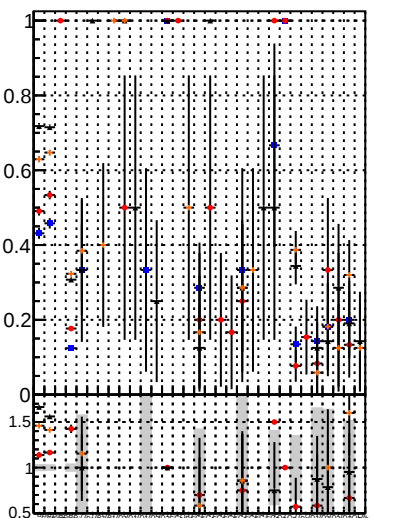
Fake rate vs. BGM SKE BDT mKFit
