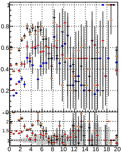
Fake rate vs. BGM SKE BDT mKFit
