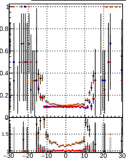
Legend for Fake rate vs v: DOM CKE BDT mKEfit BDT CKEfit
