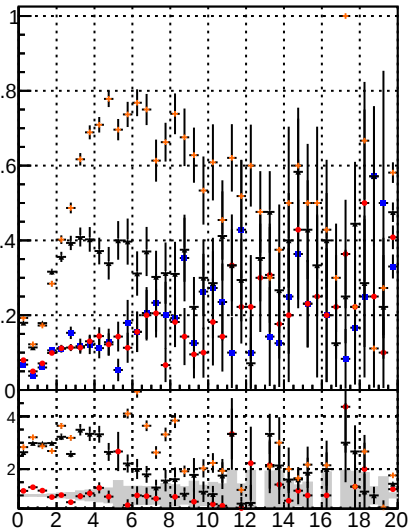
Fake rate vs. — BGM SKE — BDT mKF
