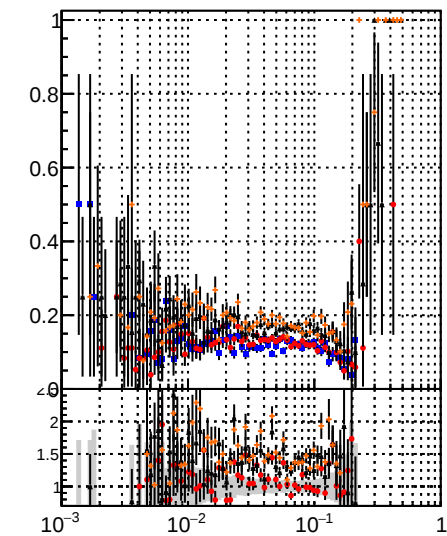
Fake rate vs \sqrt{s} DOM CKE DOM mKEfit DOM BDT mKEfit
