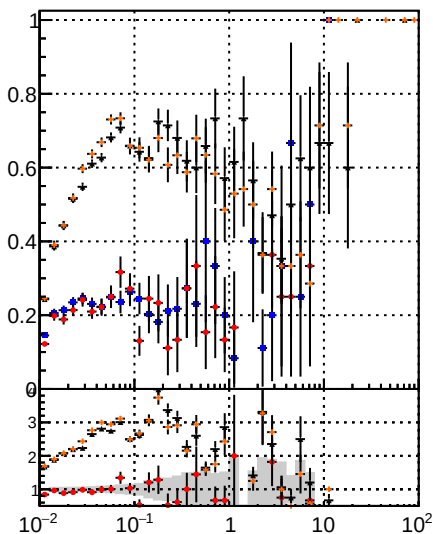
DOM CKE DOM mKEfit DOM BDT CKEfit
