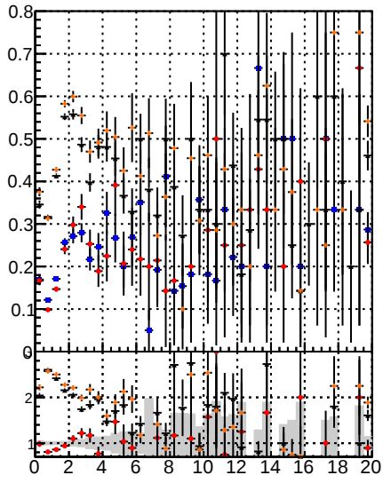
Fake rate vs. BSM SKE BDT mKF
