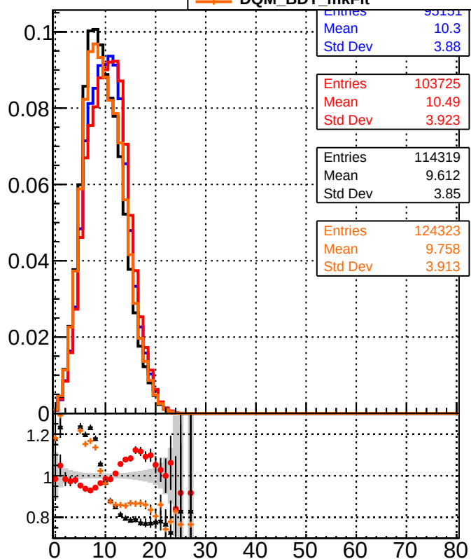
Legend for bottom row: DQM_CKF (Blue line with circles) DQM_mkFit (Red line with circles) DQM_BDT_CKF (Black line with circles) DQM_BDT_mkFit (Orange line with circles)
