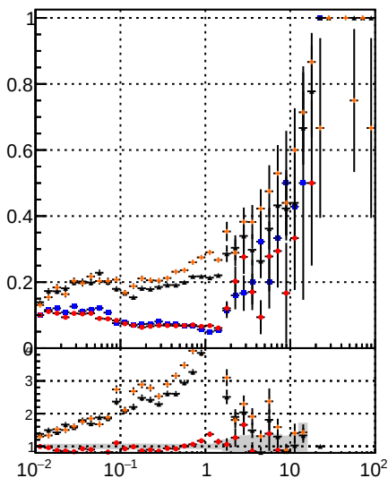
Fake rate vs v_z Legend: DOM CKE BDT mKEfit DOM BDT mKEfit
