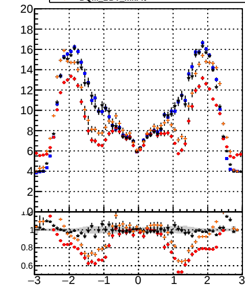
mean hit Legend: DQM_CKF (blue line), DQM_mkFit (red line), DQM_BDT_CKF (black line), DQM_BDT_mkFit (orange line)
