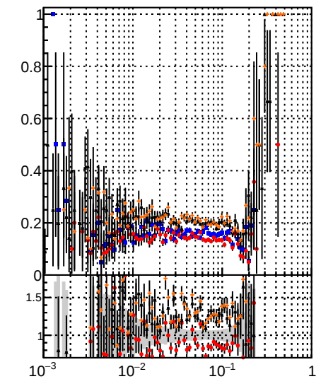
Fake rate vs \sqrt{s} Legend: DOM CKE DOM mKFit DOM BDT DOM mKFit
