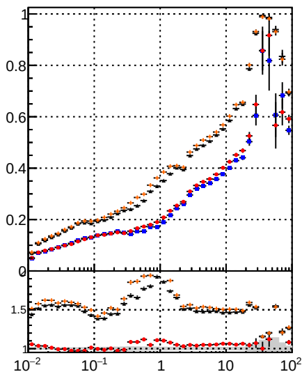
Legend for Fake rate vs v: DOM (blue squares) CKE (red circles) BDT (orange crosses) mKEfit (black dots)
