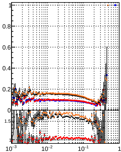
Fake rate vs \mu Legend: DOM CKE BDT mKEfit BDT CKEfit
