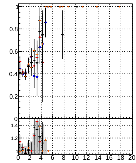
Fake rate vs. \chi^2 for BQM, SKE, BQMfit, BDT, and mKFit
