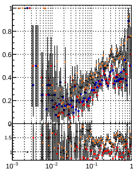
Fake rate vs \mu
