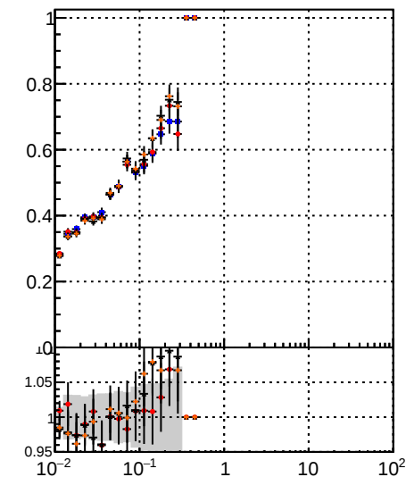
DOM CKE DOM mKEfit DOM BDT mKEfit
