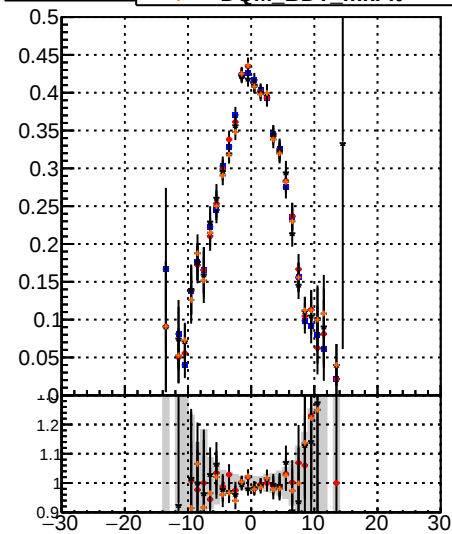
DOM CKE DOM mKEfit DOM BDT mKEfit
