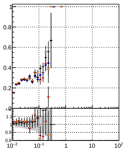
Efficiency vs. sim PV z —●— DQM_CKF —●— DQM_mkFit —●— DQM_BDT_CKF —●— DQM_BDT_mkFit
