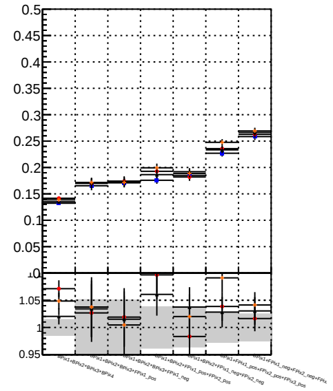
Fake rate vs. BQM SKE BQEfit BBT-mKFit
