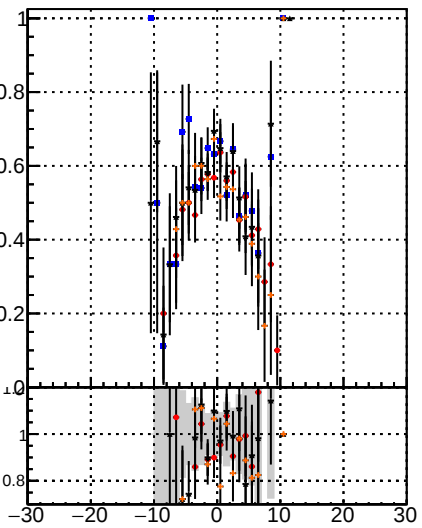
Fake rate vs v_z Legend: DOM CKE BDT mKEit DOM BDT CKEFit BDT mKEit
