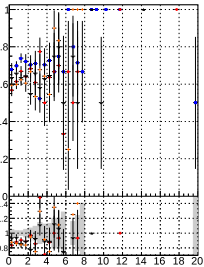
Fake rate vs. BQM SKE BQM-BDT mKFit
