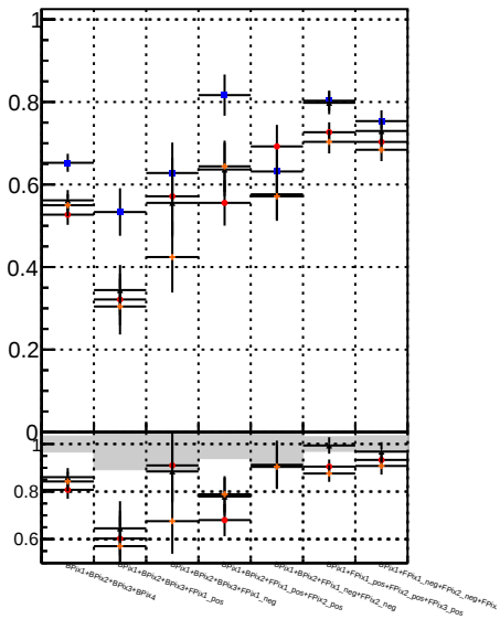
Fake rate vs. BQM SKE BQM-BDT mKFit
