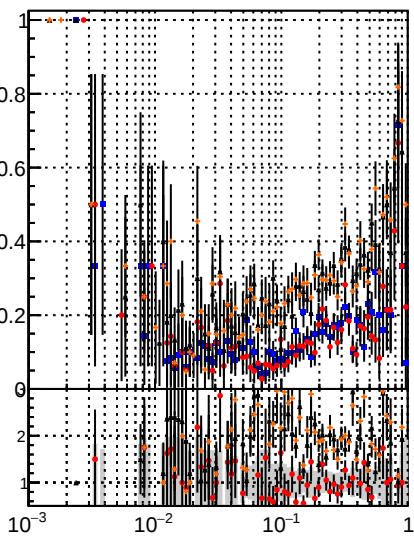
Fake rate vs \epsilon DOM CKE DOM mKEit DOM BDT CKEFit
