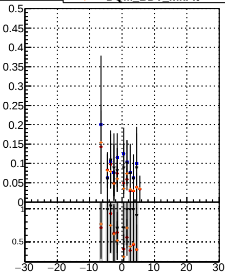
Fake rate vs v_{\text{true}} Legend: DOM (blue), CKE (red), mKFit (black), BDT (orange)
