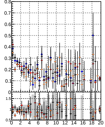
Fake rate vs. BQM SKE BQM-BDT CKE BQM-BDT-mKFit
