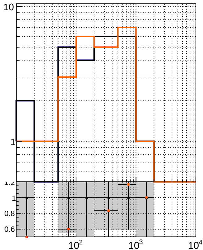
RecoAssoc2GenPVMatchedNotHighest_Pt2
