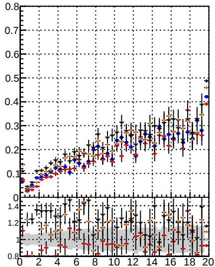
Fake rate vs. Model Color Shape BSM Blue Circle SKE Orange Circle BDT Black Circle mKF Red Circle
