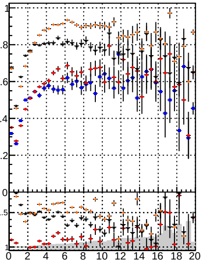
Fake rate vs. BDT SKE BDT+CKE BDT+mKE
