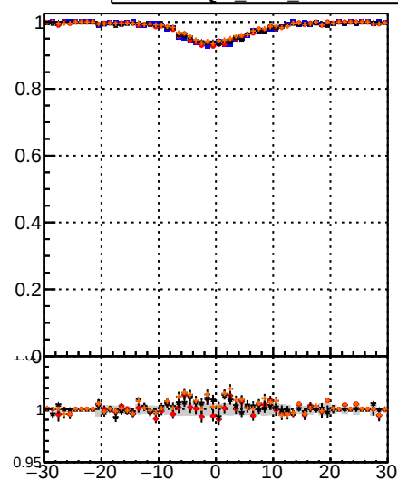
Fake rate vs v_z Legend: DOM (blue squares) CKE (red crosses) mKEit (black dots) BDT (orange triangles) CKEit (green circles) mKEit (black dots)
