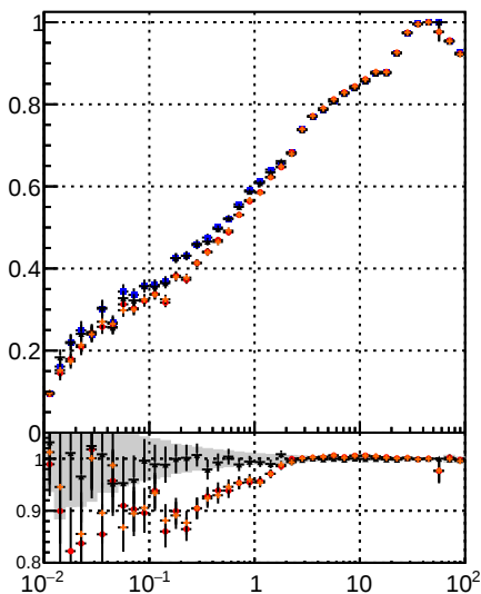
Legend for Fake rate vs vertpos: DOM (blue circles) CKE (orange circles) mKEit (red circles) BDT (black circles)
