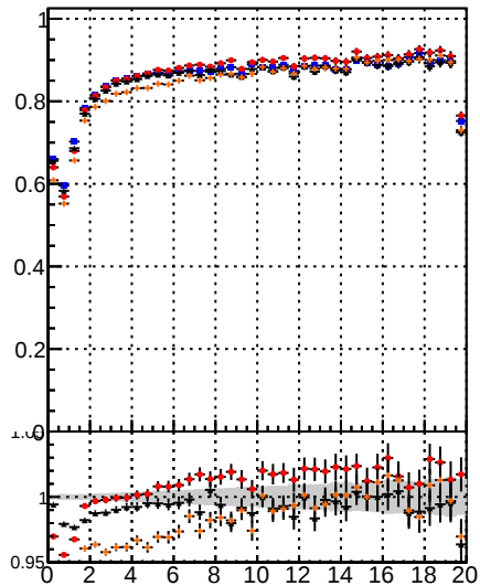
Fake rate vs. BSM-SKE BSM-SKEfit BSM-BDT BSM-BDT-mKF
