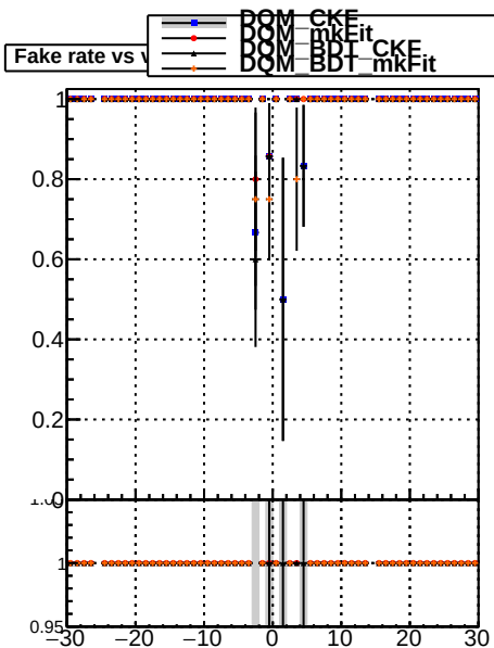
Fake rate vs. sim PV z
