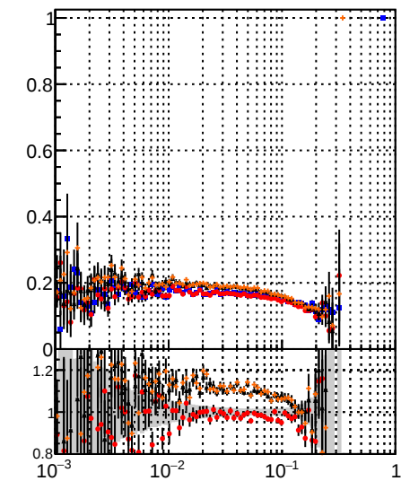
Fake rate vs \epsilon Legend: DOM CKE BDT mkFit BDT CKE BDT mkFit
