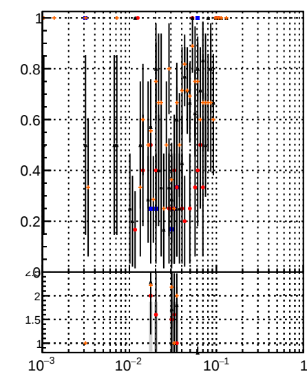
Fake rate vs dr Legend: DOM (black line) CKE (blue line) BDT (red line) mkFit (orange line)
